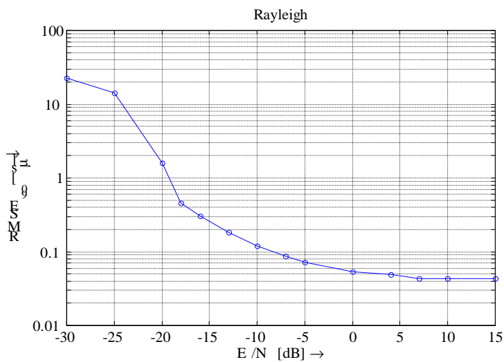
Figure V.4.5. TOA estimation error (in \mu s ) as function of E_b/N_0 in a flat Rayleigh fading channel.
