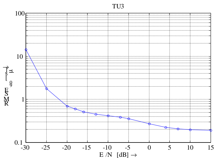
Figure V.4.8. TOA estimation error (in μs) as function of E_b/N_0 in a TU3 channel.
