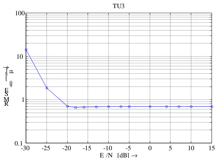
Figure V.4.9. TOA estimation error (in μs) as function of E_b/N_0 in a TU3 channel without multipath rejection.
