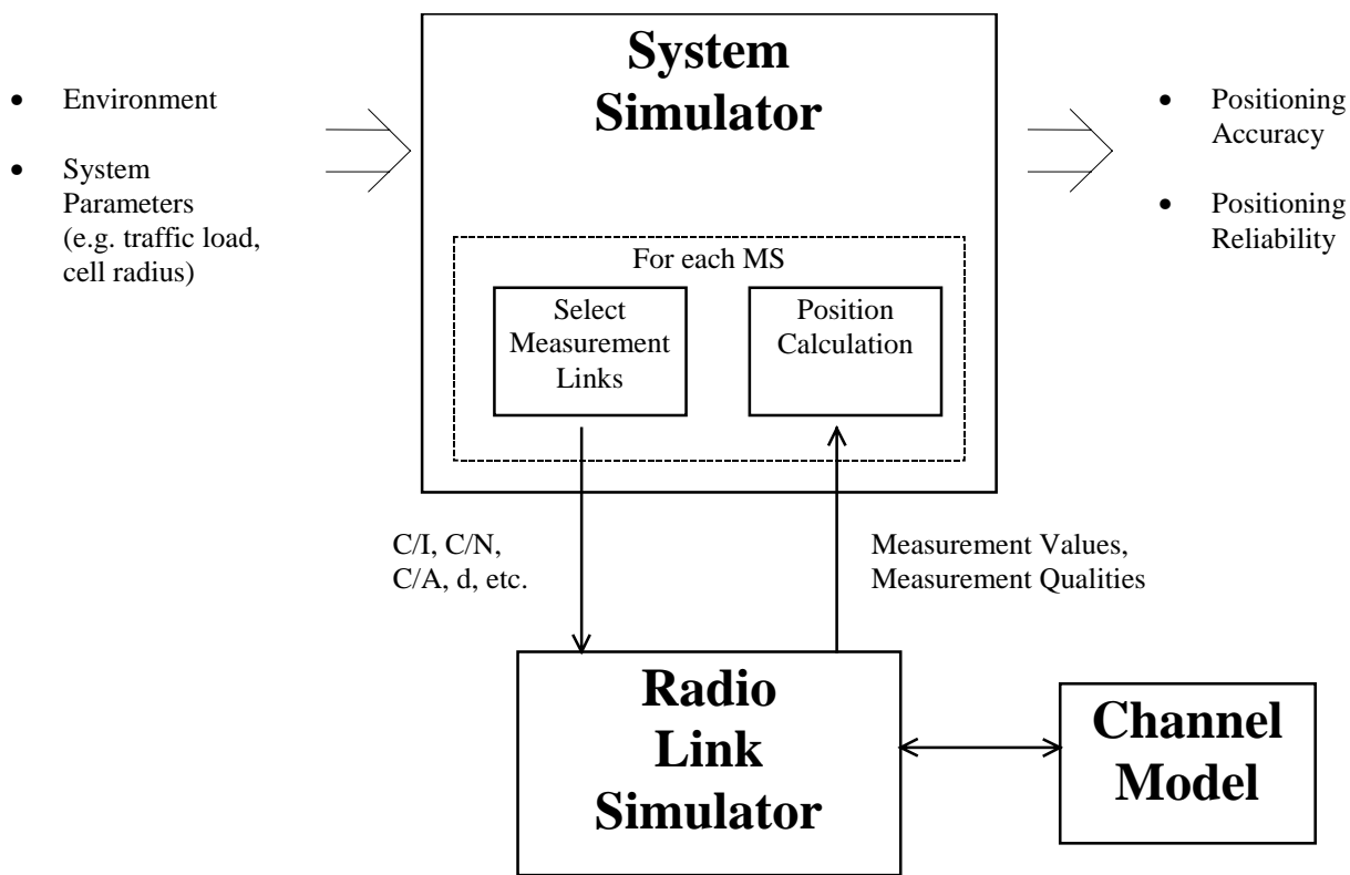
Figure 2.1. Positioning Simulator
